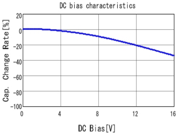
■ GRM033R71C222KA88 C-DC bias capchange, 25.0degC, AC1.
