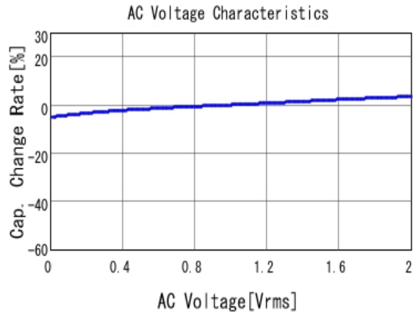
■ GRM033R71C222KA88 C-AC Voltage capchange, DCOV, 25.0d
