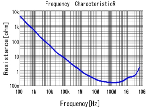
■ GRM033R71C222KA88 R DCOV, 25degC
