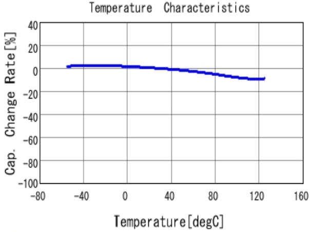
■ GRM033R71C222KA88 C-Temp. capchange, DCO. 0V, AC1.0Vrm
