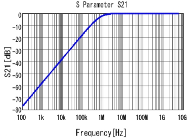
■ GRM033R71C222KA88 S21 DCOV, 25degC
