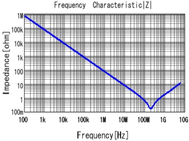
■ GRM033R71C222KA88 |Z| DCOV, 25degC
