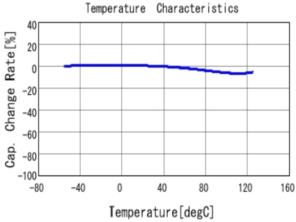
■ GRM033R71C102KA01 C-Temp. capchange, DCO. 0V, AC1.0V rm
