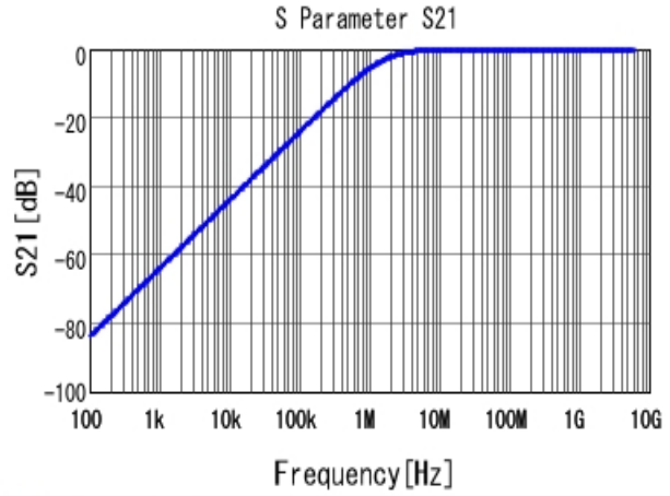
■ GRM033R71C102KA01 S21 DCOV, 25degC
