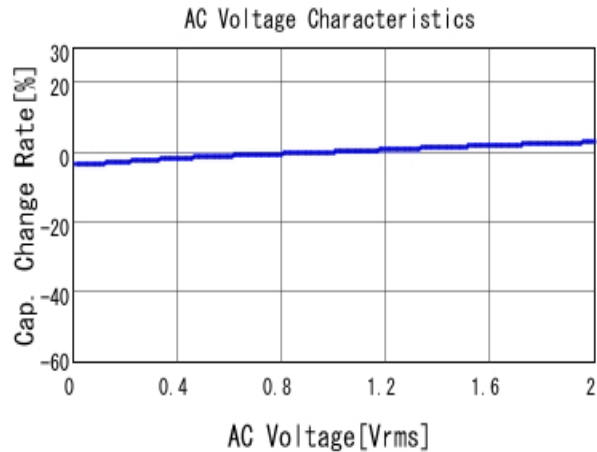
■ GRM033R71C102KA01 C-AC Voltage capchange, DCOV, 25.0d
