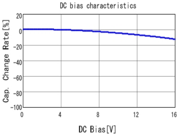
■ GRM033R71C102KA01 C-DC bias capchange, 25.0degC, AC1.
