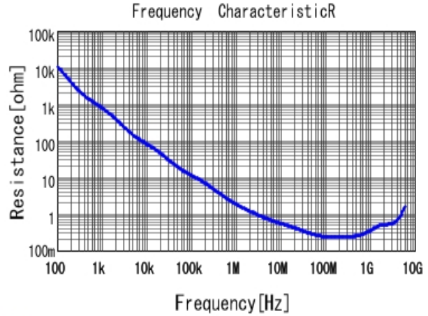
■ GRM033R71C102KA01 R DCOV, 25degC
