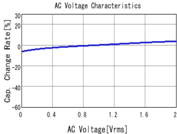
■ GRM033R71A103KA01 C-AC Voltage capchange, DCOV, 25.0d
