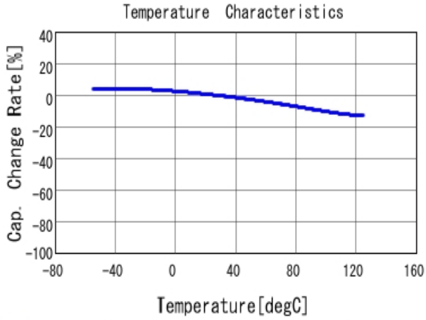
■ GRM033R71A103KA01 C-Temp. capchange, DCO. 0V, AC1.0V rm
