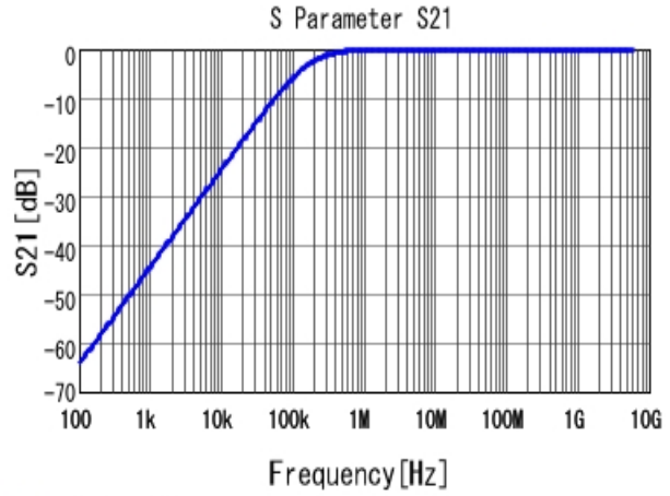
■ GRM033R71A103KA01 S21 DCOV, 25degC
