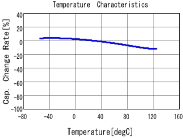
■ GRM033R70J472KA01 C-Temp. capchange, DCO. 0V, AC1.0V r m
