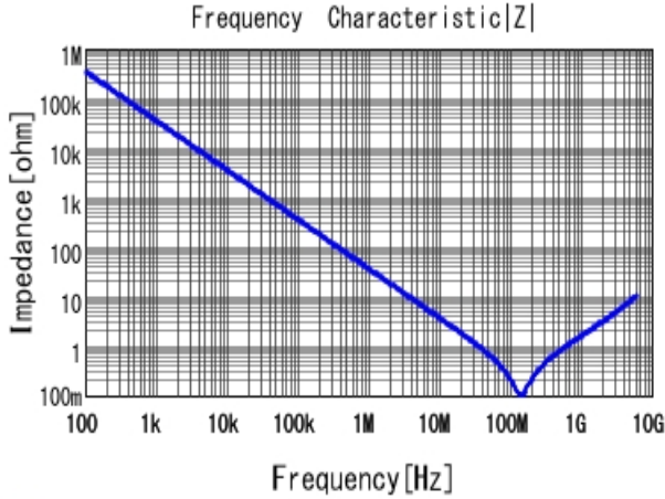
■ GRM033R70J472KA01 |Z| DCOV, 25degC
