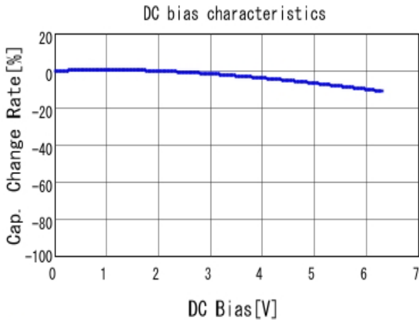
■ GRM033R70J472KA01 C-DC bias capchange, 25.0degC, AC1.
