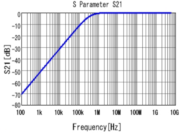
■ GRM033R70J472KA01 S21 DCOV, 25degC
