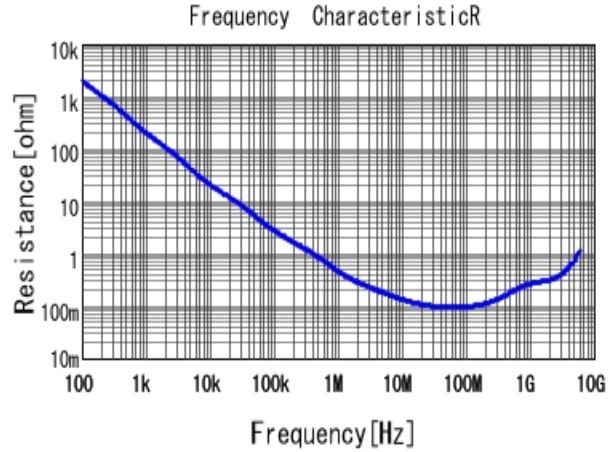
■ GRM033R70J472KA01 R DCOV, 25degC
