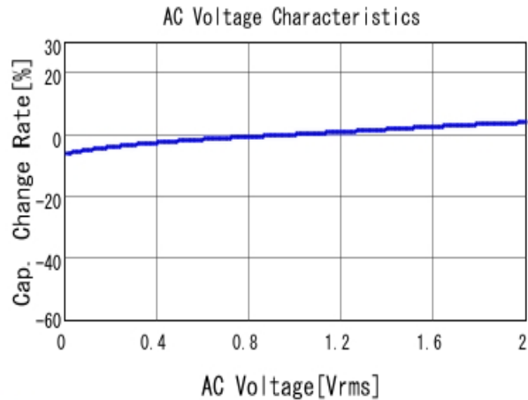
■ GRM033R70J472KA01 C-AC Voltage capchange, DCOV, 25.0d
