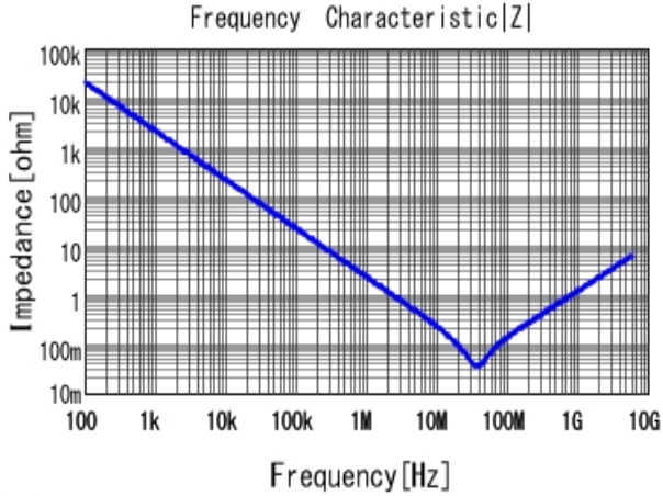
■ GRM033R61E104ME14 |Z| DCOV, 25degC
