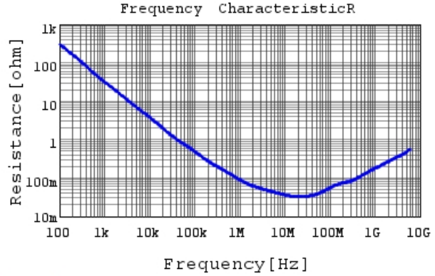
GRM033R61E104KE14 R DCOV,25degC
