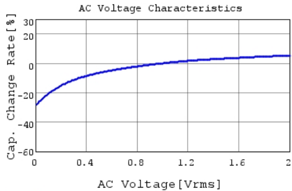
GRM033R61E104KE14 C-AC Voltage capchange, Dc
