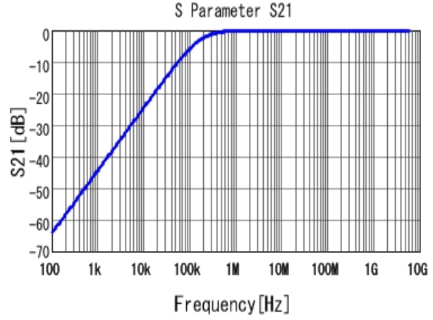
■ GRM033R61E103KA12 S21 DCOV, 25degC
