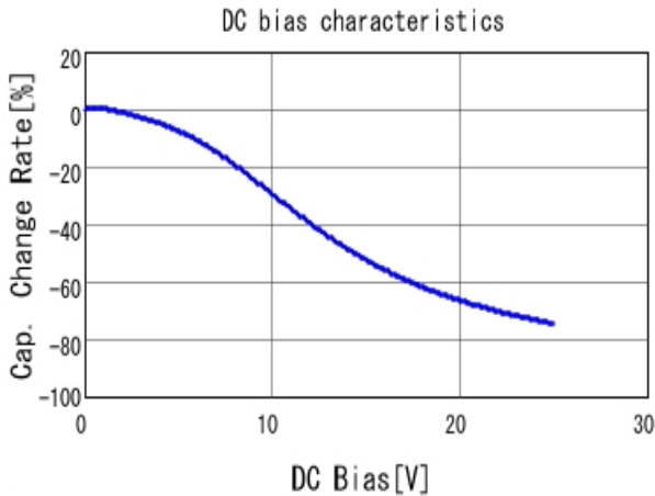
■ GRM033R61E103KA12 C-DC bias capchange, 25.0degC, AC1.
