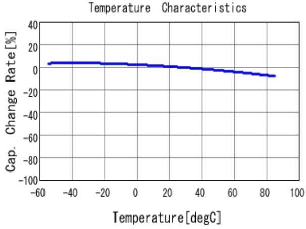
■ GRM033R61E103KA12 C-Temp. capchange, DCO. 0V, AC1.0V rm
