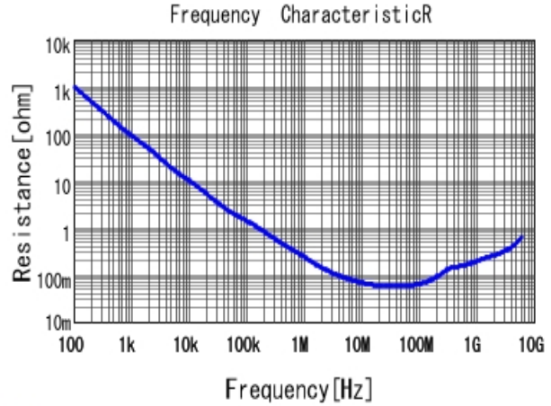
■ GRM033R61E103KA12 R DCOV, 25degC
