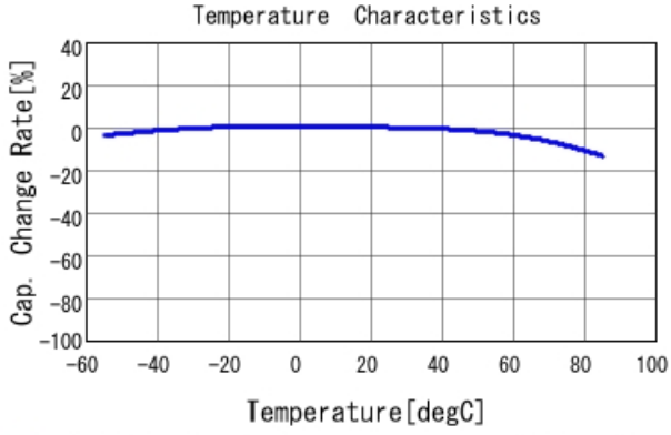
■ GRM033R61A225KE47 C-Temp. capchange, DCO. 0V, ACO. 2Vrm
