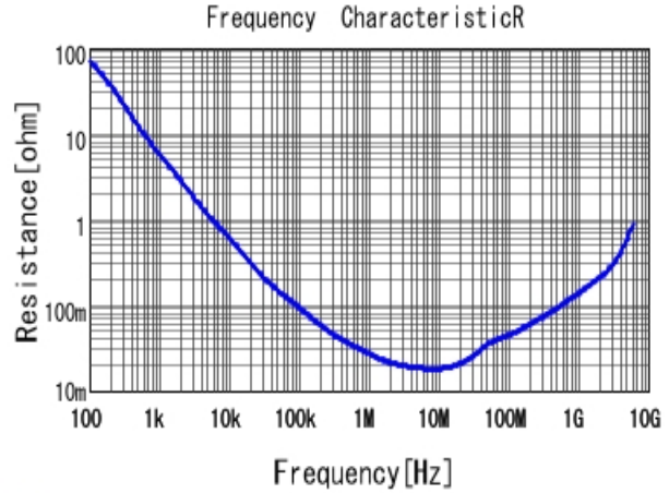
■ GRM033R61A224KE90 R DCOV, 25degC
