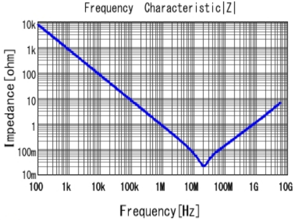
■ GRM033R61A224KE90 |Z| DCOV, 25degC
