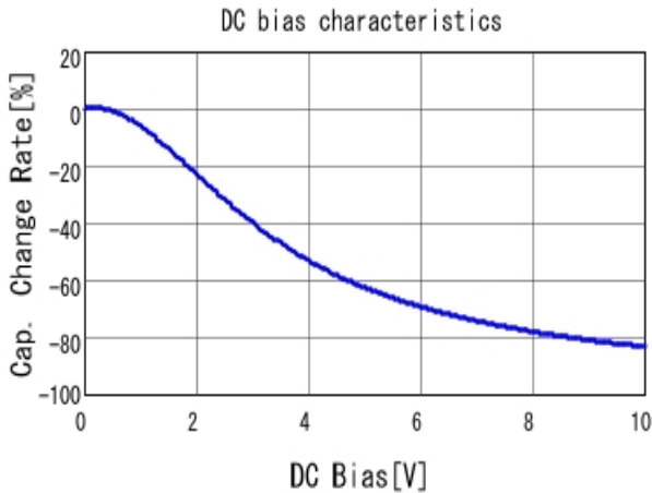
■ GRM033R61A224KE90 C-DC bias capchange, 25.0degC, AC0.
