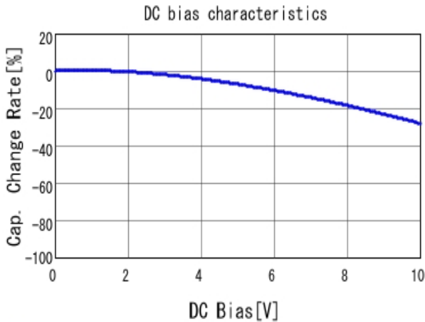
■ GRM033R61A103KA01 C-DC bias capchange, 25.0degC, AC1.
