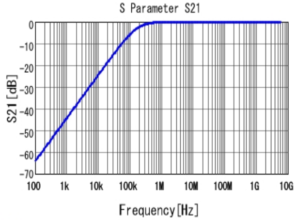
■ GRM033R61A103KA01 S21 DCOV, 25degC
