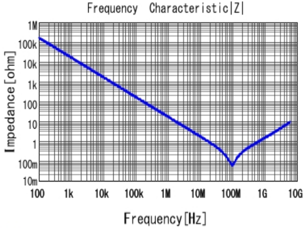
■ GRM033R61A103KA01 |Z| DCOV, 25degC
