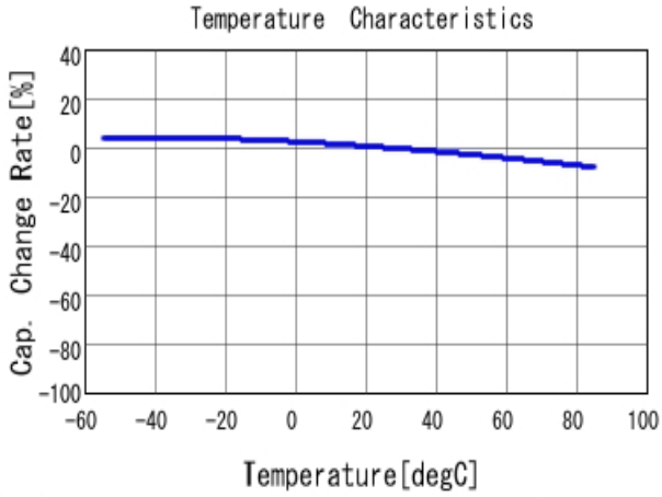
■ GRM033R61A103KA01 C-Temp. capchange, DCO. 0V, AC1.0V rm
