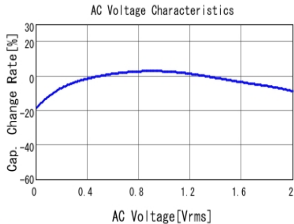
■ GRM033R60J474KE90 C-AC Voltage capchange, DCOV, 25.0d
