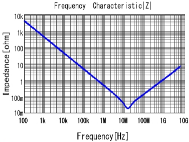
■ GRM033R60J474KE90 |Z| DCOV, 25degC
