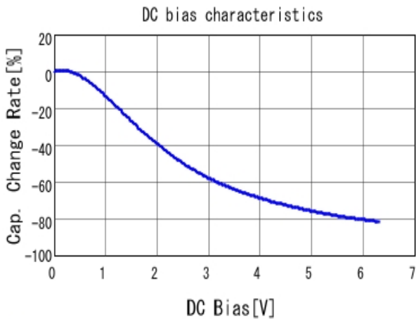
■ GRM033R60J474KE90 C-DC bias capchange, 25.0degC, AC0.
