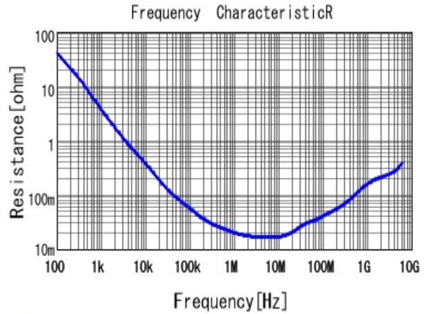
■ GRM033R60J474KE90 R DCOV, 25degC
