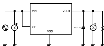
Circuit ③
