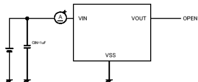
Circuit ③
