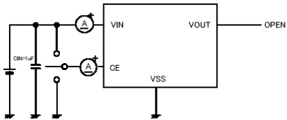
Circuit ②
