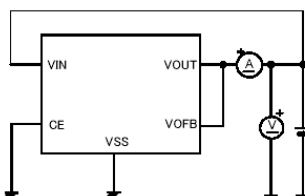
Circuit ④
