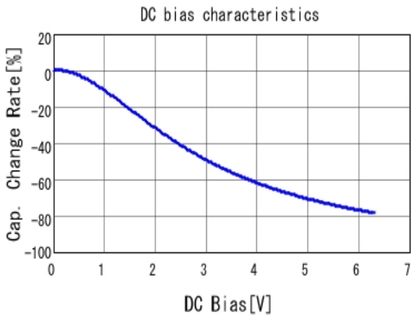
■ GRM033R60J224KE15 C-DC bias capchange, 25.0degC, AC0.
