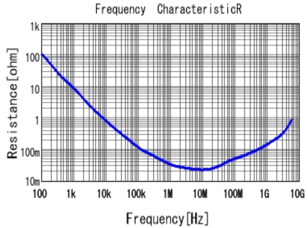
■ GRM033R60J224KE15 R DCOV, 25degC
