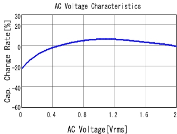
■ GRM033R60J224KE15 C-AC Voltage capchange, DCOV, 25.0d
