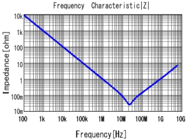
■ GRM033R60J224KE15 |Z| DCOV, 25degC
