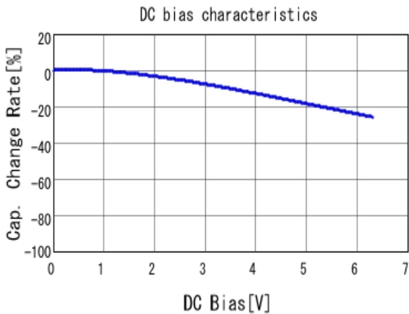
■ GRM033R60J153KE01 C-DC bias capchange, 25.0degC, AC0.
