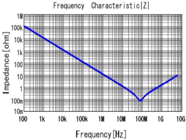
■ GRM033R60J153KE01 |Z| DCOV, 25degC
