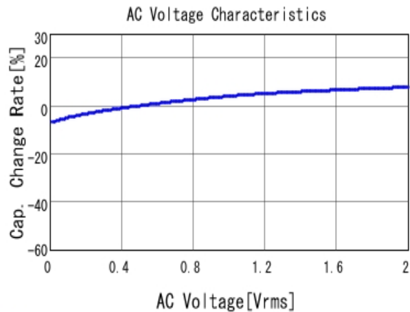
■ GRM033R60J153KE01 C-AC Voltage capchange, DCOV, 25.0d
