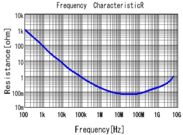
■ GRM033R60J153KE01 R DCOV, 25degC
