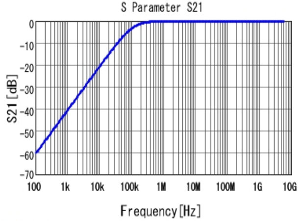
■ GRM033R60J153KE01 S21 DCOV, 25degC
