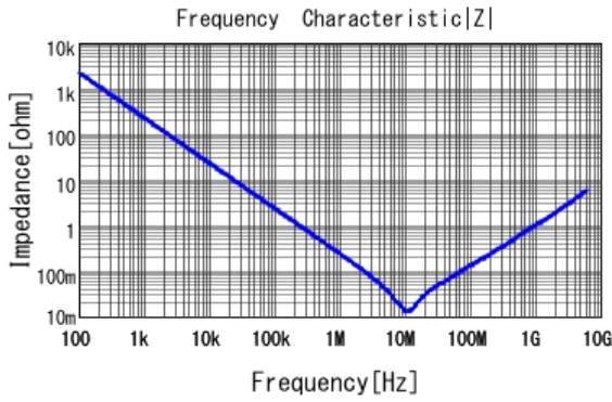
■ GRM033R60J105MEA2 |Z| DCOV, 25degC
