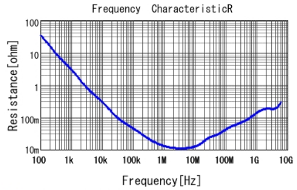
■ GRM033R60J105MEA2 R DCOV, 25degC
