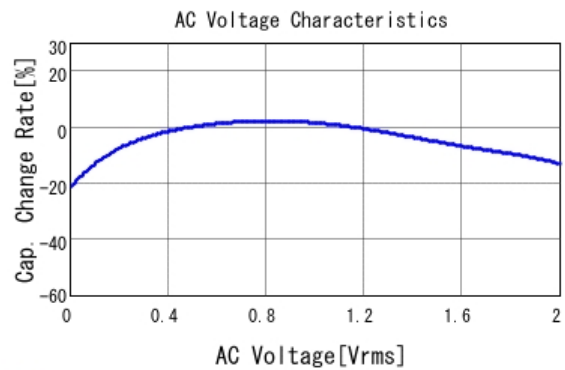
■ GRM033R60J105MEA2 C-AC Voltage capchange, DCOV, 25.0d
