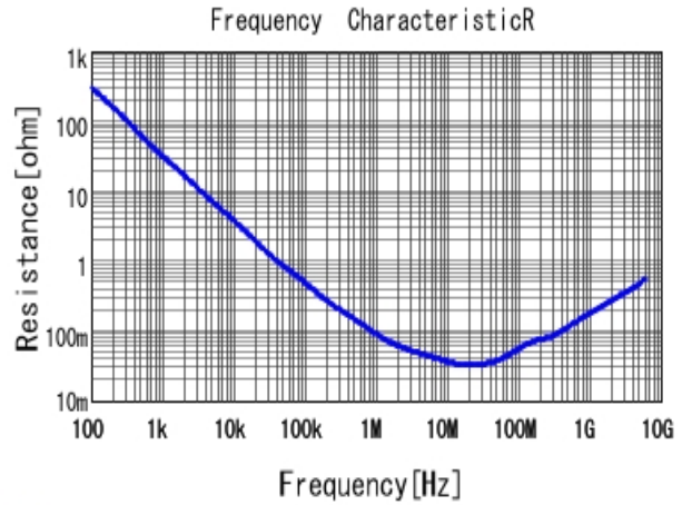
■ GRM033C71A104KE14 R DCOV, 25degC
