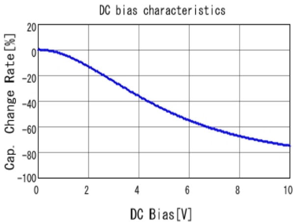
■ GRM033C71A104KE14 C-DC bias capchange, 25.0degC, AC1V
