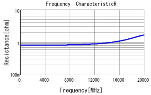
■ GRM0335C1HR80WA01 R DCOV, 25degC
