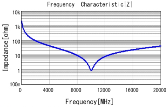
■ GRM0335C1HR80WA01 |Z| DCOV, 25degC
