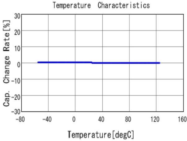
■ GRM0335C1HR30WA01 C-Temp. capchange, DCOV, AC1Vrms
