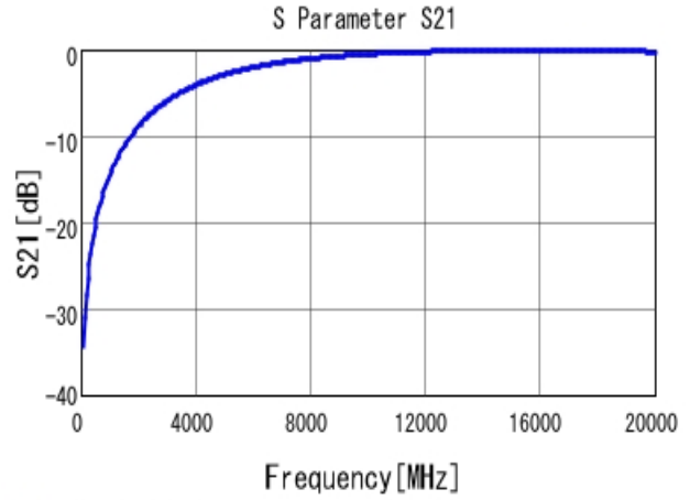
■ GRM0335C1HR30WA01 S21 DCOV, 25degC
