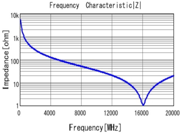
■ GRM0335C1HR30WA01 |Z| DC0V, 25degC
