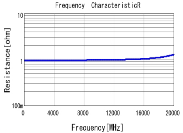
■ GRM0335C1HR30WA01 R DC0V, 25degC
