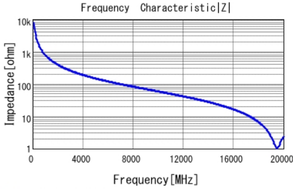
■ GRM0335C1HR20BA01 |Z| DCOV, 25degC
