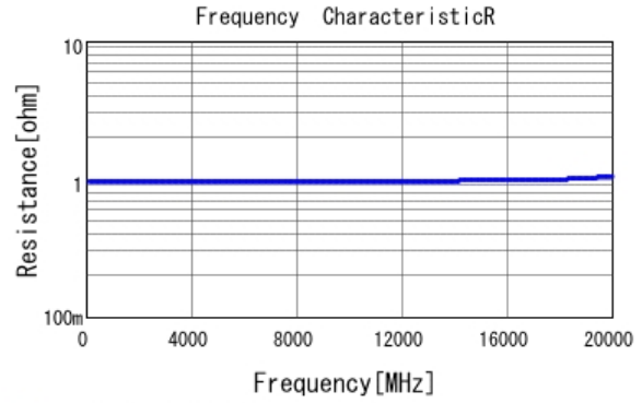
■ GRM0335C1HR20BA01 R DCOV, 25degC
