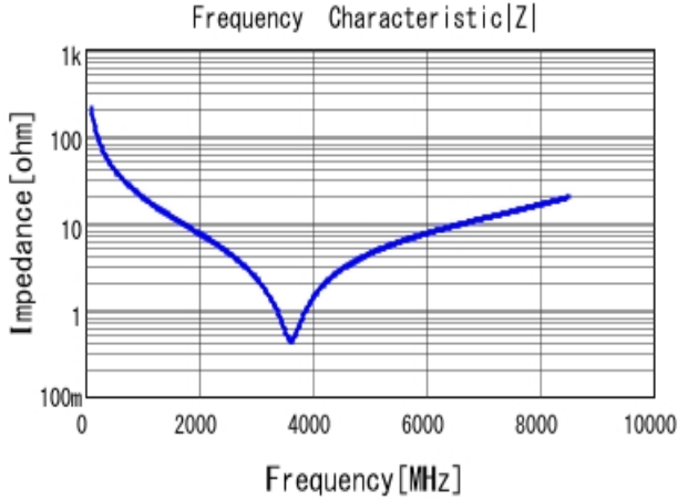
■ GRM0335C1H7R5BA01 |Z| DC0V, 25degC
