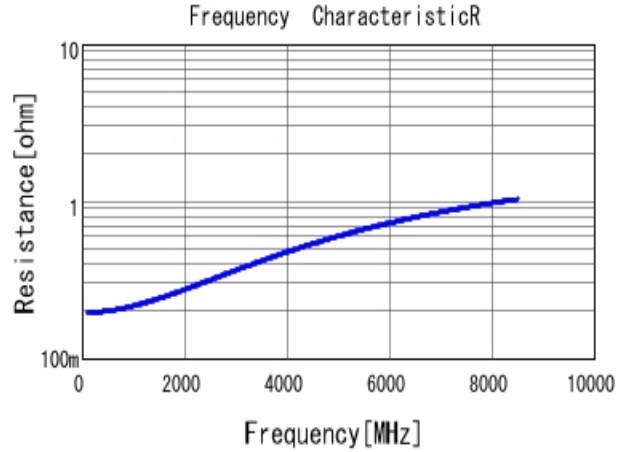
■ GRM0335C1H7R5BA01 R DC0V, 25degC
