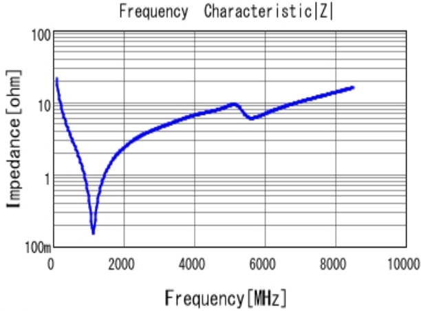
■ GRM0335C1H750JA01 |Z| DC0V, 25degC
