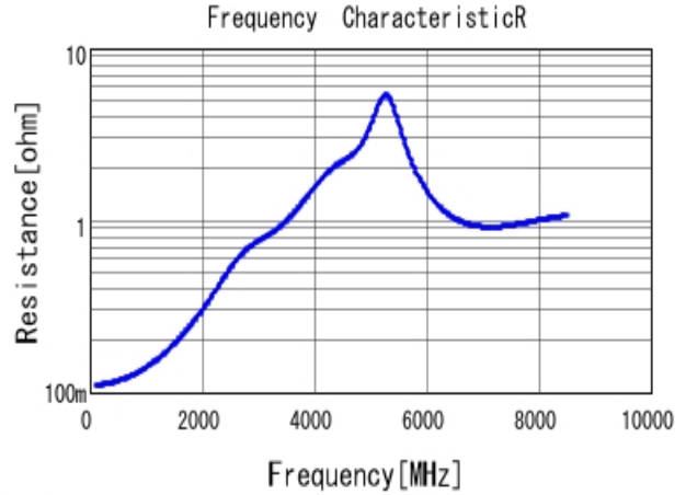
■ GRM0335C1H750JA01 R DC0V, 25degC
