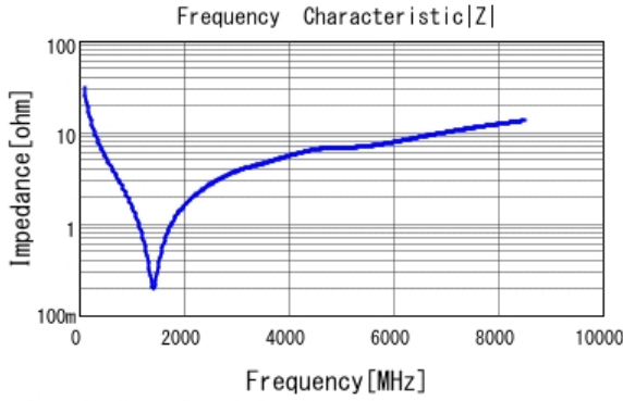
■ GRM0335C1H510GA01 |Z| DCOV, 25degC
