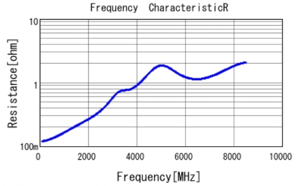
■ GRM0335C1H510GA01 R DCOV, 25degC
