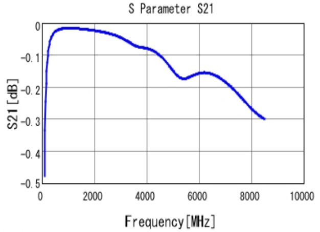
■ GRM0335C1H470JA01 S21 DCOV, 25degC
