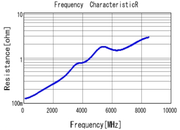
■ GRM0335C1H470JA01 R DC0V, 25degC
