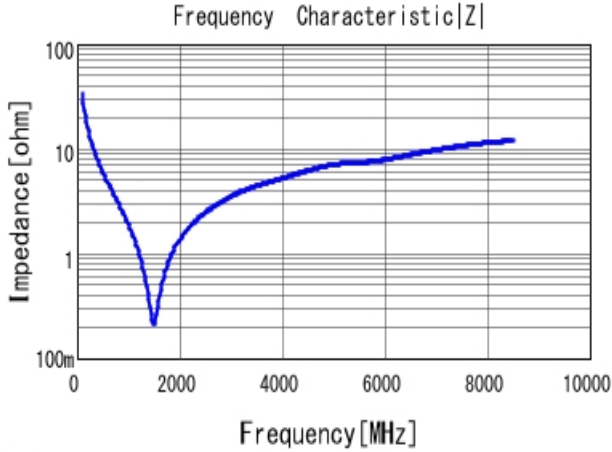
■ GRM0335C1H470JA01 |Z| DC0V, 25degC
