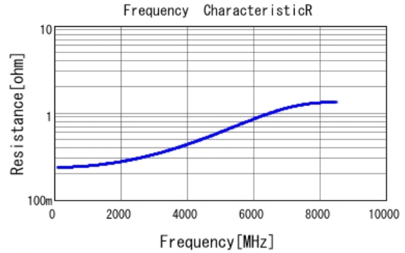
■ GRM0335C1H3R9BA01 R DCOV, 25degC
