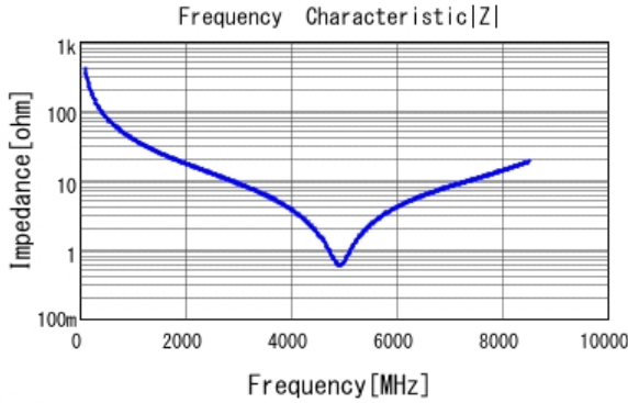
■ GRM0335C1H3R9BA01 |Z| DCOV, 25degC
