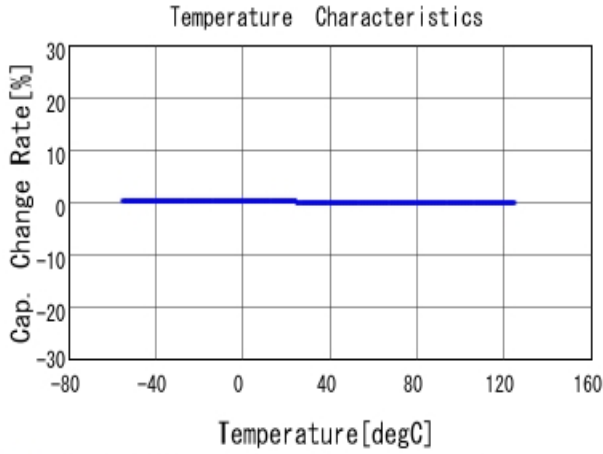
■ GRM0335C1H1R0CA01 C-Temp. capchange, DCOV, AC1Vrms
