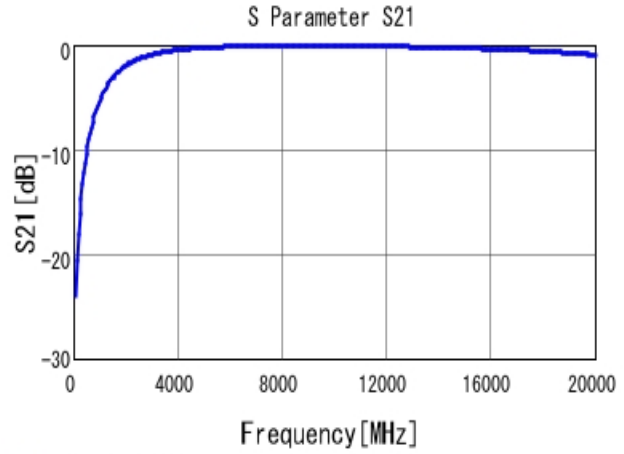
■ GRM0335C1H1R0CA01 S21 DCOV, 25degC
