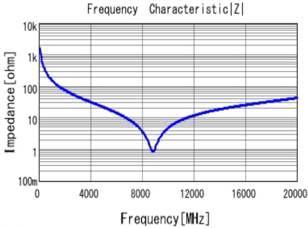
■ GRM0335C1H1R0CA01 |Z| DC0V, 25degC
