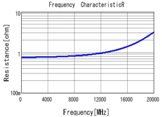
■ GRM0335C1H1R0CA01 R DC0V, 25degC
