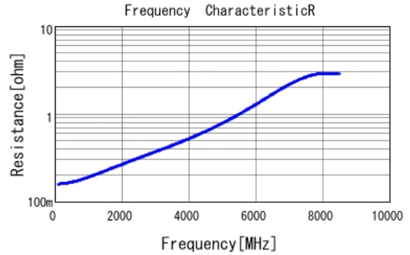
■ GRM0335C1H180GA01 R DCOV, 25degC
