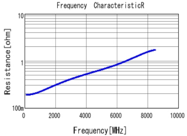
■ GRM0335C1H120JA01 R DC0V, 25degC
