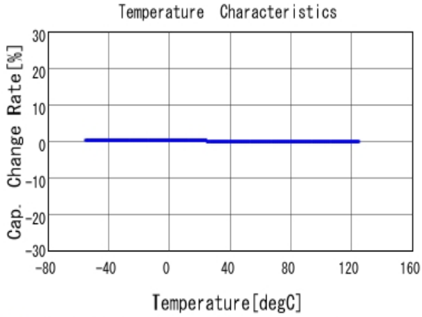
■ GRM0335C1H120JA01 C-Temp. capchange, DCOV, AC1Vrms
