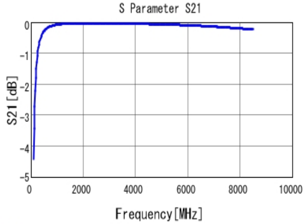
■ GRM0335C1H120JA01 S21 DCOV, 25degC
