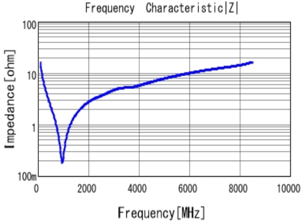
■ GRM0335C1H101JA01 |Z| DC0V, 25degC
