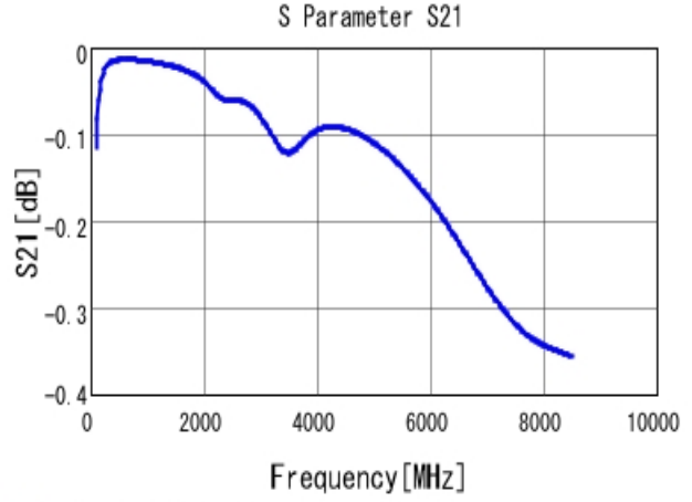
■ GRM0335C1H101JA01 S21 DCOV, 25degC
