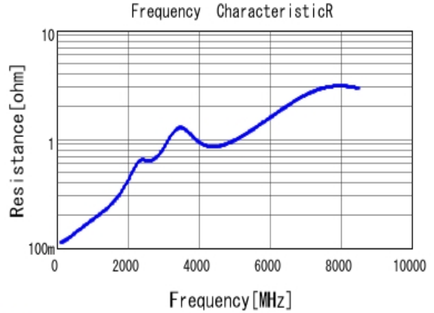
■ GRM0335C1H101JA01 R DC0V, 25degC
