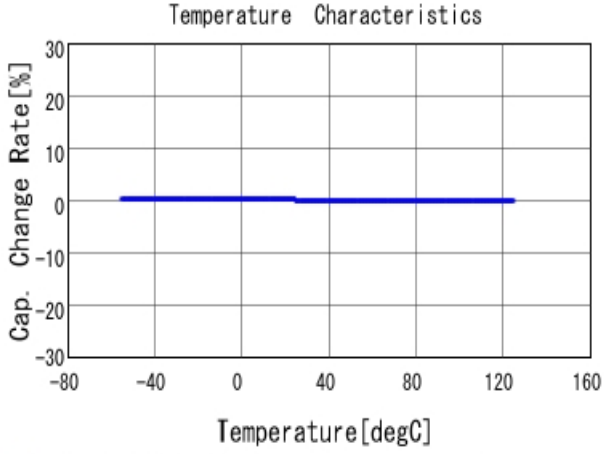
■ GRM0335C1H101JA01 C-Temp. capchange, DCOV, AC1Vrms
