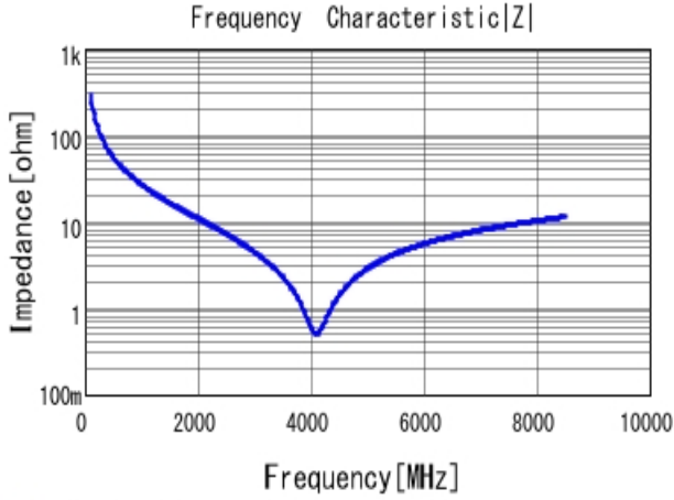
■ GRM0335C1E5R6BA01 |Z| DC0V, 25degC
