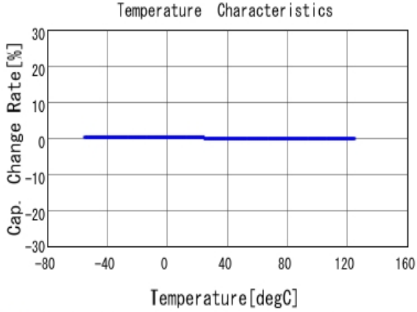
■ GRM0335C1E5R6BA01 C-Temp. capchange, DCOV, AC1Vrms
