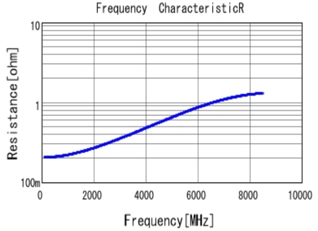
■ GRM0335C1E5R6BA01 R DC0V, 25degC
