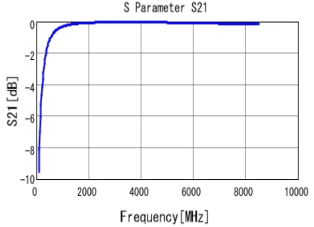
■ GRM0335C1E5R6BA01 S21 DCOV, 25degC
