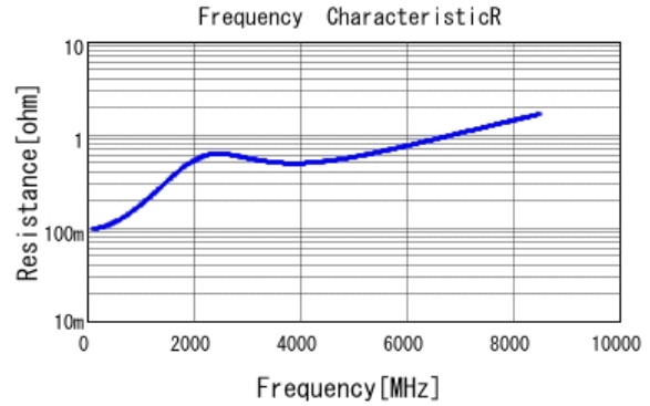
■ GRM0335C1E271JA01 R DCOV, 25degC
