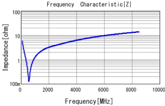
■ GRM0335C1E271JA01 |Z| DCOV, 25degC
