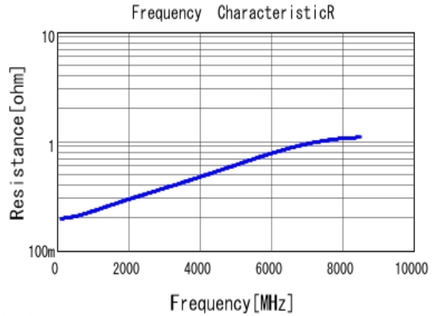
■ GRM0335C1E100JA01 R DC0V, 25degC
