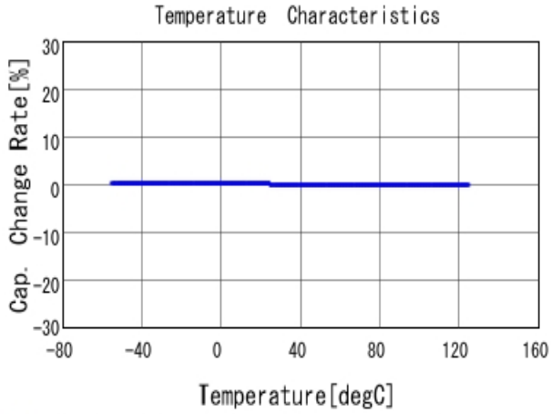
■ GRM0335C1E100JA01 C-Temp. capchange, DCOV, AC1Vrms
