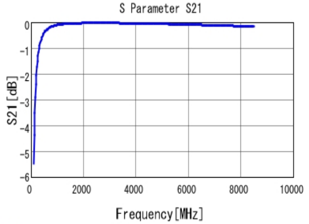
■ GRM0335C1E100JA01 S21 DCOV, 25degC
