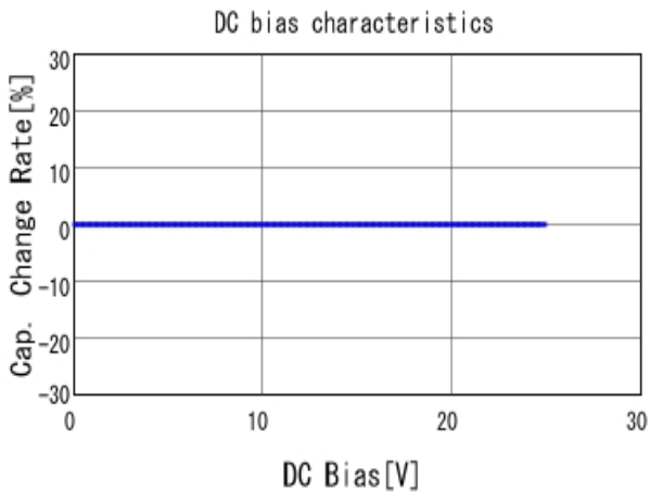
■ GRM0335C1E100JA01 C-DC bias capchange, 25.0degC, AC1V
