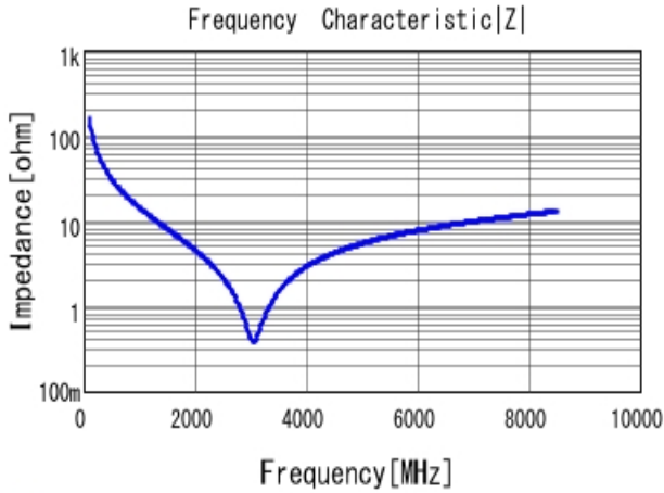
■ GRM0335C1E100JA01 |Z| DC0V, 25degC
