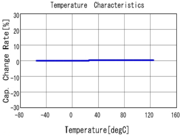
■ GRM0225C1H1R5WA03 C-Temp. capchange, DCOV, AC1Vrms
