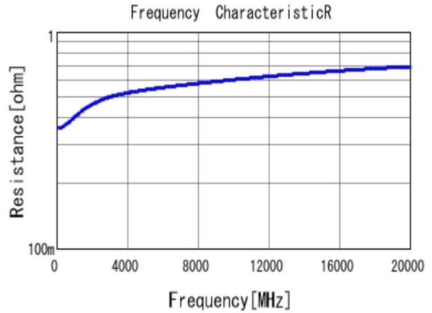
■ GRM0225C1H1R5WA03 R DC0V, 25degC
