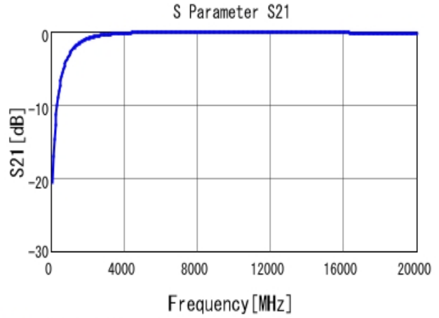
■ GRM0225C1H1R5WA03 S21 DCOV, 25degC
