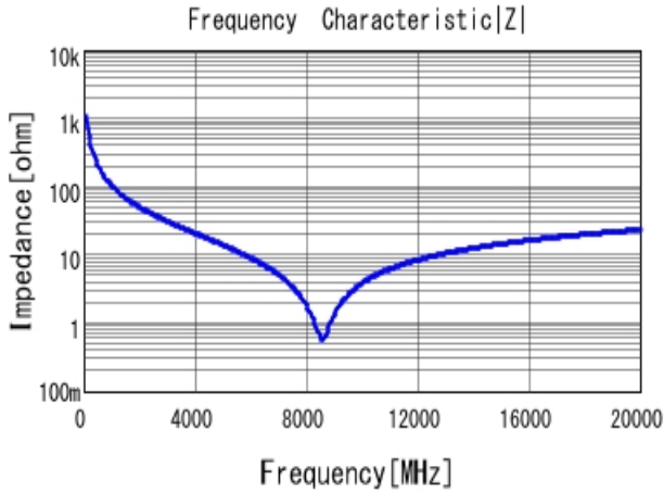
■ GRM0225C1H1R5WA03 |Z| DC0V, 25degC
