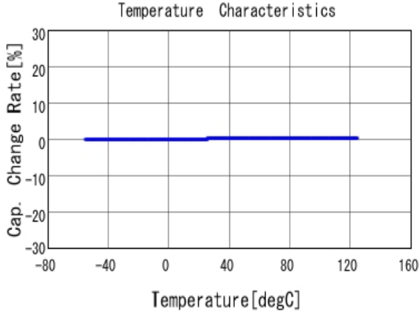
■ GRM0225C1E8R0BA03 C-Temp. capchange, DCOV, AC1Vrms
