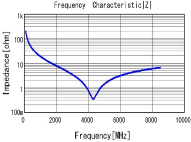
■ GRM0225C1E8R0BA03 |Z| DC0V, 25degC
