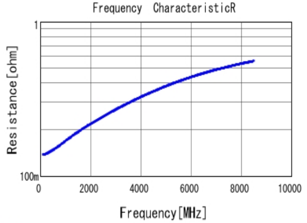
■ GRM0225C1E8R0BA03 R DC0V, 25degC
