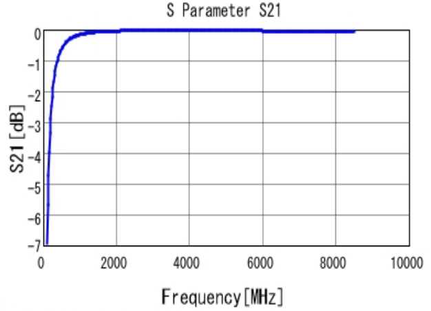
■ GRM0225C1E8R0BA03 S21 DCOV, 25degC
