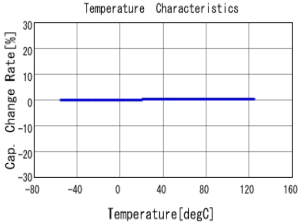
■ GRM0222C1H330JA02 C-Temp. capchange, DCOV, AC1Vrms
