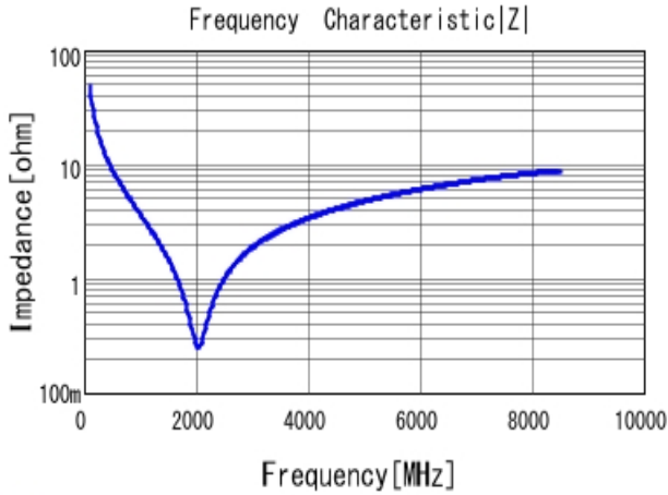
■ GRM0222C1H330JA02 |Z| DC0V, 20degC
