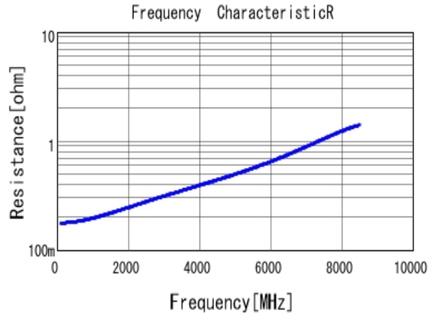
■ GRM0222C1H330JA02 R DC0V, 20degC
