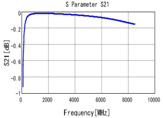
■ GRM0222C1H330JA02 S21 DCOV, 20degC
