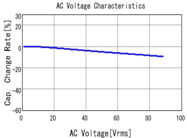
■ GRJ43DR72E474KWJ1 C-AC Voltage capchange, DC0V, 25.0d
