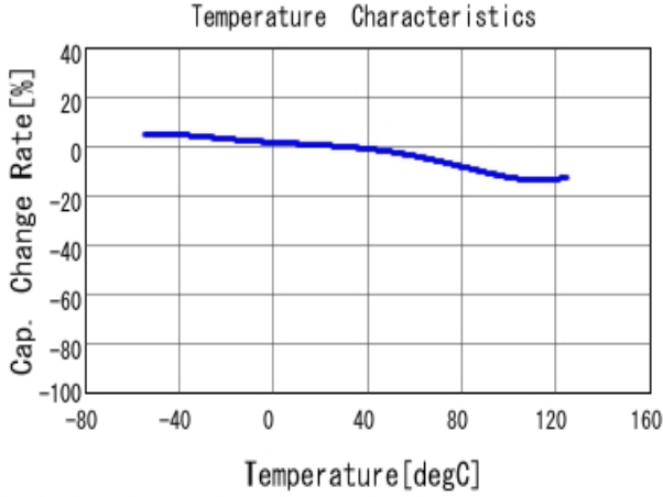
■ GRJ43DR72E474KWJ1 C-Temp. capchange, DCOV, AC1Vrms
