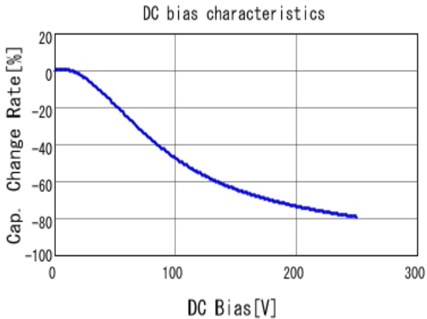
■ GRJ43DR72E474KWJ1 C-DC bias capchange, 25.0degC, AC1V
