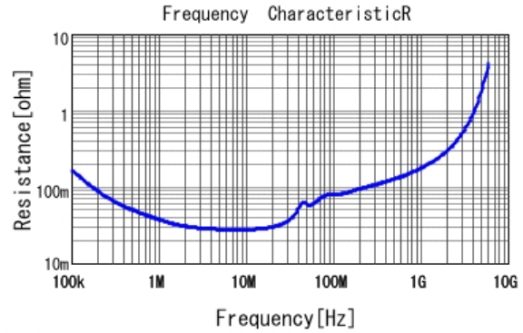
■ GRJ188R72A104KE11 R DC0V, 25degC
