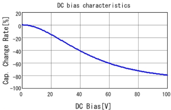
■ GRJ188R72A104KE11 C-DC bias capchange, 25.0degC, AC1.
