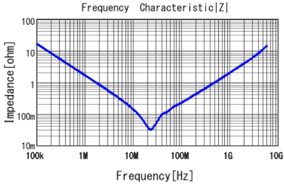
■ GRJ188R72A104KE11 |Z| DC0V, 25degC
