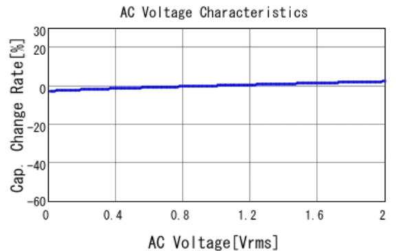
■ GRJ188R72A104KE11 C-AC Voltage capchange, DC0V, 25.0d
