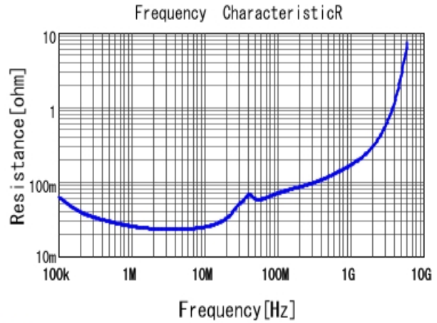
■ GRJ188R71H224KE11 R DCOV, 25degC
