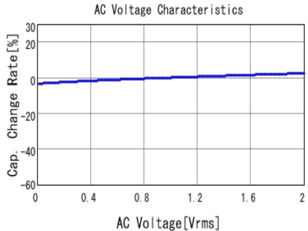
■ GRJ188R71H224KE11 C-AC Voltage capchange, DCOV, 25.0d
