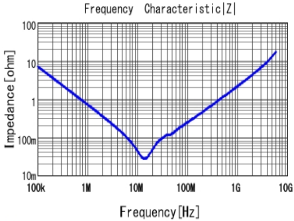
■ GRJ188R71H224KE11 |Z| DCOV, 25degC
