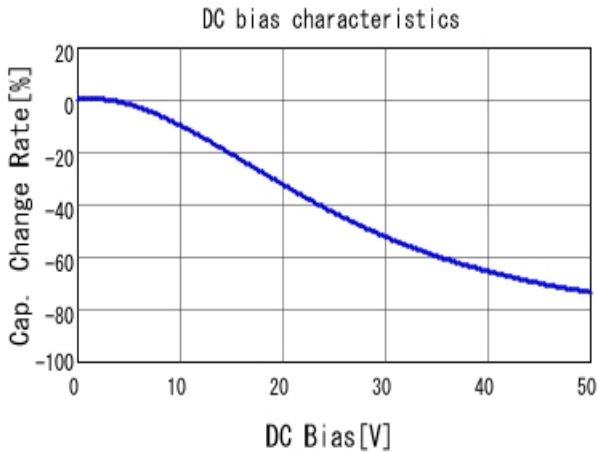
■ GRJ188R71H224KE11 C-DC bias capchange, 25.0degC, AC1.
