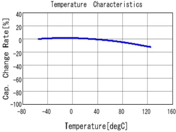
■ GRJ188R71H224KE11 C-Temp. capchange, DCO. 0V, AC1.0V r m
