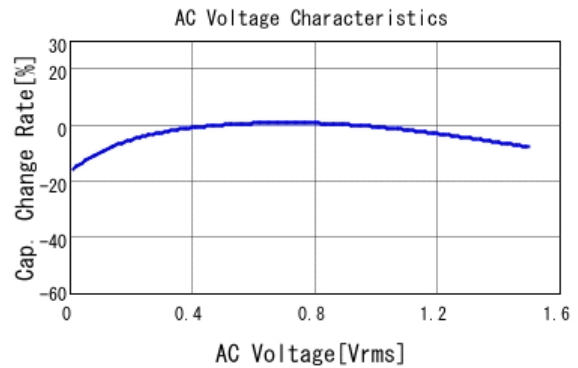
■ GRJ155R60J106ME11 C-AC Voltage capchange, DCOV, 25.0d
