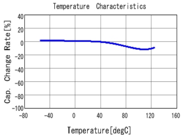
■ GR443QR73D222KW01 C-Temp. capchange, DCOV, AC1Vrms
