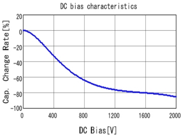
■ GR443QR73D222KW01 C-DC bias capchange, 25.0degC, AC1V
