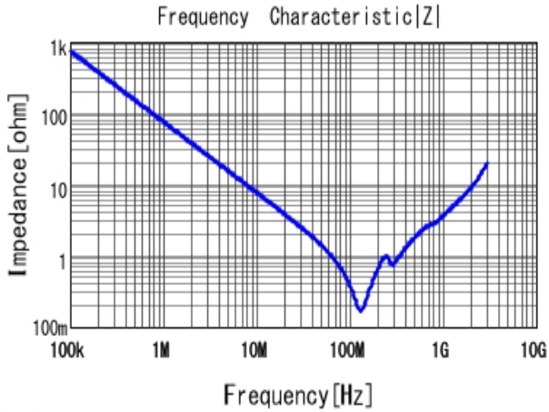
■ GR443QR73D222KW01 |Z| DCOV, 25degC
