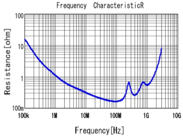
■ GR443QR73D222KW01 R DCOV, 25degC
