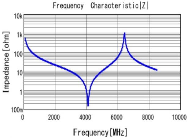
■ GQM22M5C2H3R0CB01 |Z| DC0V, 25degC
