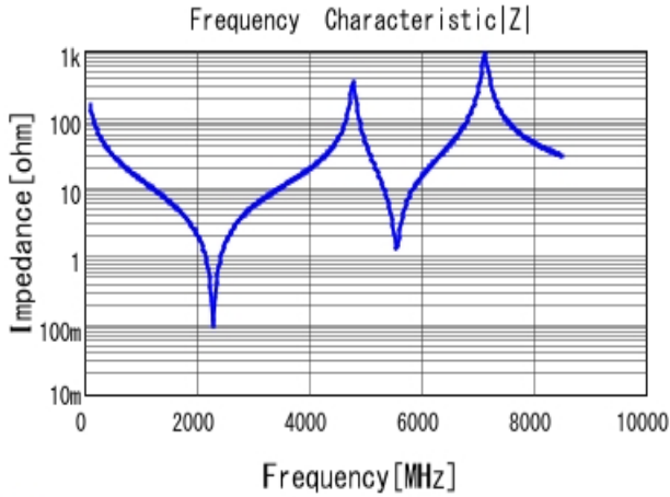
■ GQM22M5C2H100JB01 |Z| DC0V, 25degC
