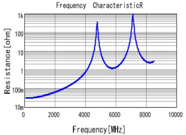
■ GQM22M5C2H100JB01 R DC0V, 25degC
