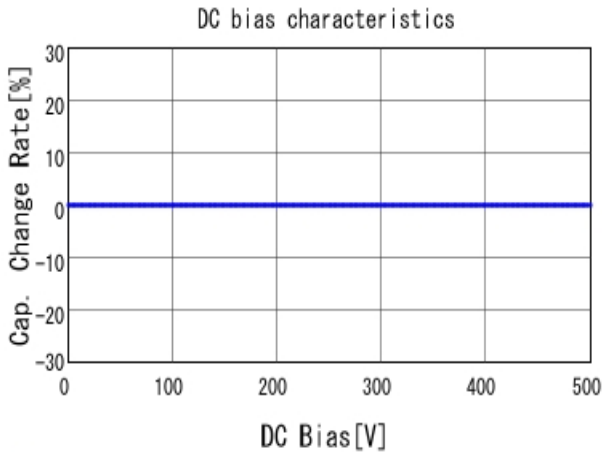
■ GQM22M5C2H100JB01 C-DC bias capchange, 25.0degC, AC1V
