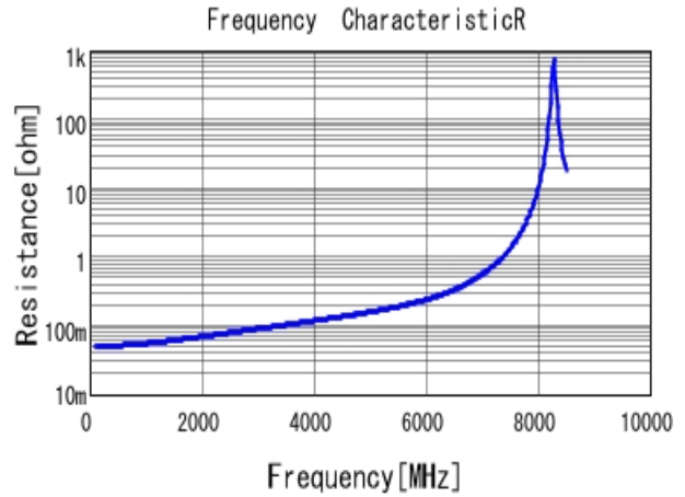
■ GQM2195C2E3R3BB12 R DC0V, 25degC
