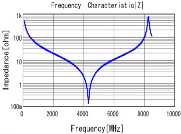
■ GQM2195C2E3R3BB12 |Z| DC0V, 25degC
