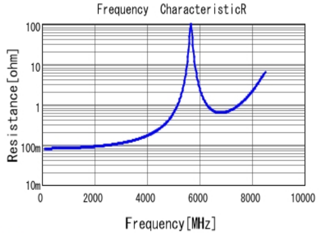
■ GQM1875C2E100JB12 R DC0V, 25degC
