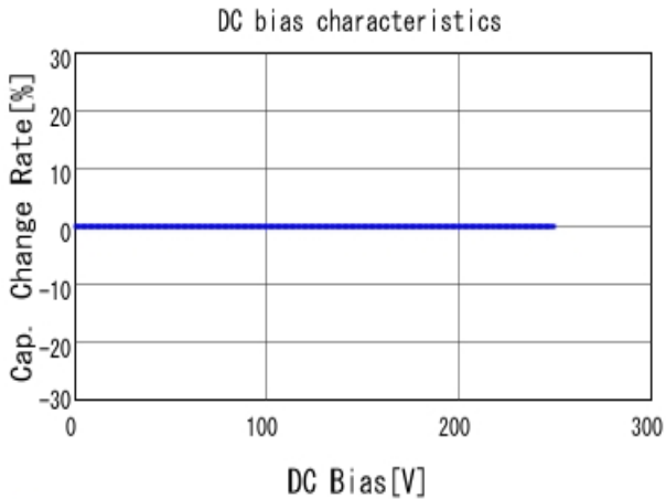
■ GQM1875C2E100JB12 C-DC bias capchange, 25.0degC, AC1V
