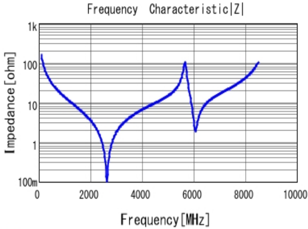
■ GQM1875C2E100JB12 |Z| DC0V, 25degC
