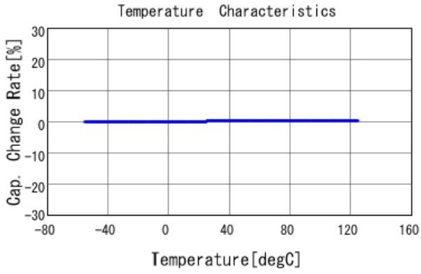
GJM1555C1HR90WB01 C-Temp. capchange, DCOV, AC1Vrms
