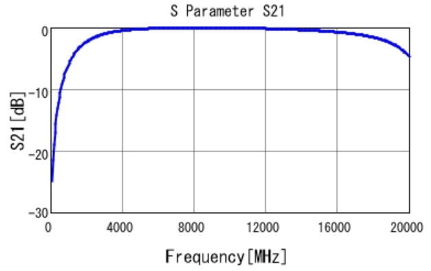
GJM1555C1HR90WB01 S21 DCOV, 25degC
