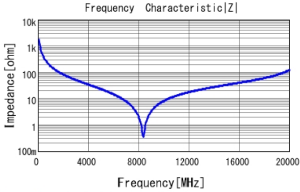
GJM1555C1HR90WB01 |Z| DCOV, 25degC
