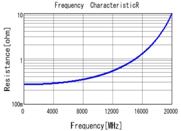
■ GJM1555C1HR80WB01 R DC0V, 25degC
