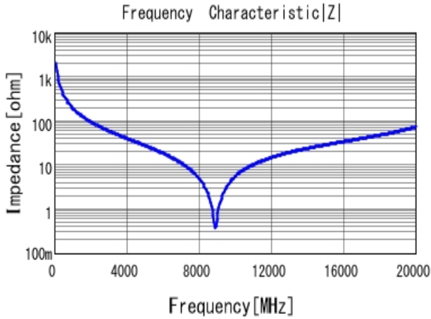
■ GJM1555C1HR80WB01 |Z| DC0V, 25degC
