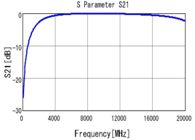
■ GJM1555C1HR80WB01 S21 DCOV, 25degC
