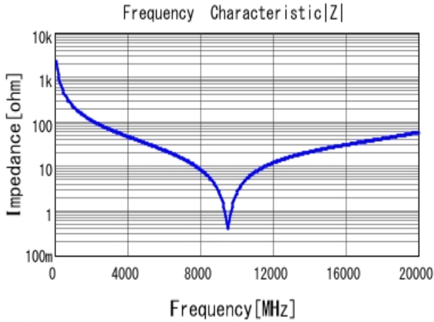
GJM1555C1HR70BB01 |Z| DC0V, 25degC
