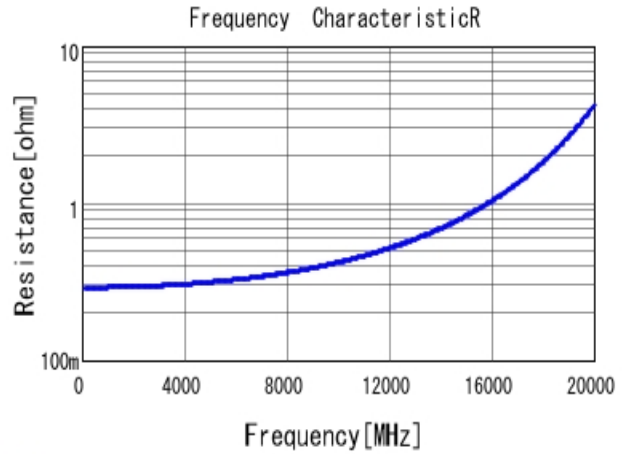
GJM1555C1HR70BB01 R DC0V, 25degC
