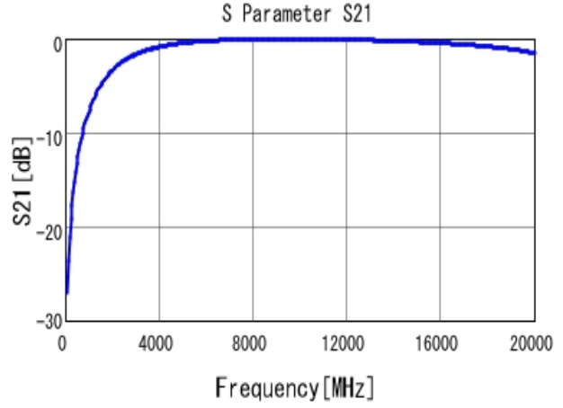
■ GJM1555C1HR70BB01 S21 DCOV, 25degC
