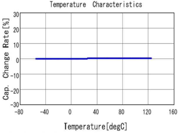
■ GJM1555C1HR70BB01 C-Temp. capchange, DCOV, AC1Vrms
