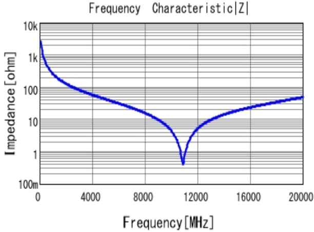
GJM1555C1HR60BB01 |Z| DC0V, 25degC
