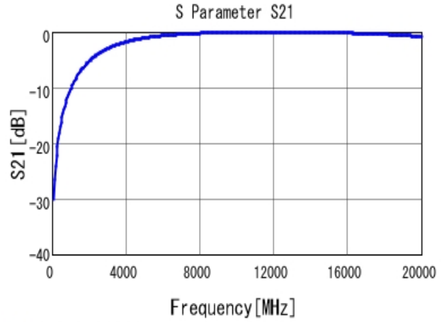
■ GJM1555C1HR50WB01 S21 DCOV, 25degC
