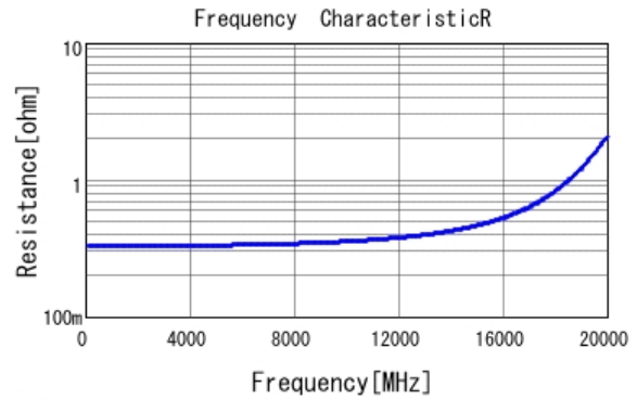
■ GJM1555C1HR50BB01 R DCOV, 25degC
