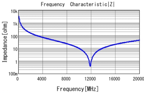
■ GJM1555C1HR50BB01 |Z| DCOV, 25degC
