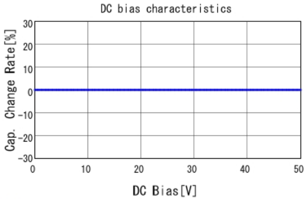
GJM1555C1HR30WB01 C-DC bias capchange, 25.0degC, AC1V
