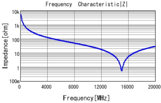
GJM1555C1HR30WB01 |Z| DC0V, 25degC
