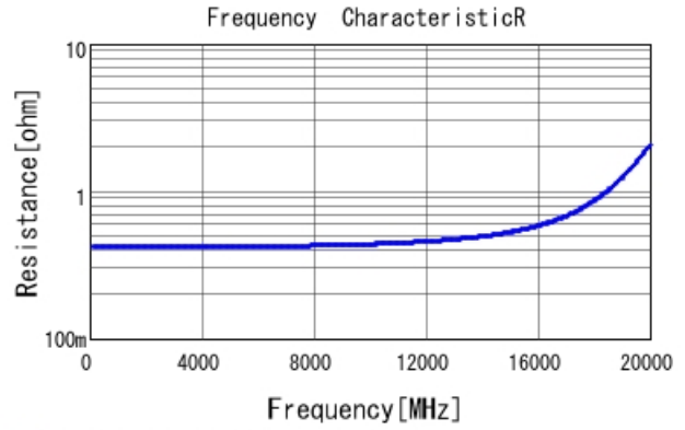
GJM1555C1HR30WB01 R DC0V, 25degC
